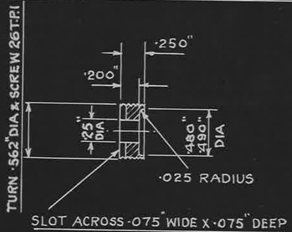
BUSH - PART 2
