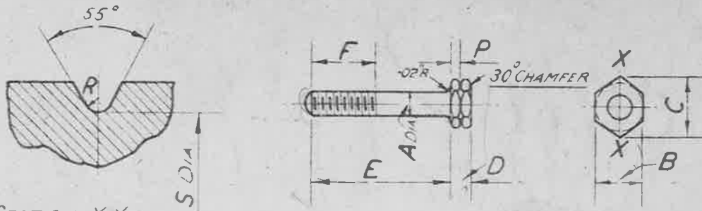
PART SECTION X X (ENLARGED)
