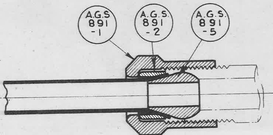
METAL PIPE JOINT
