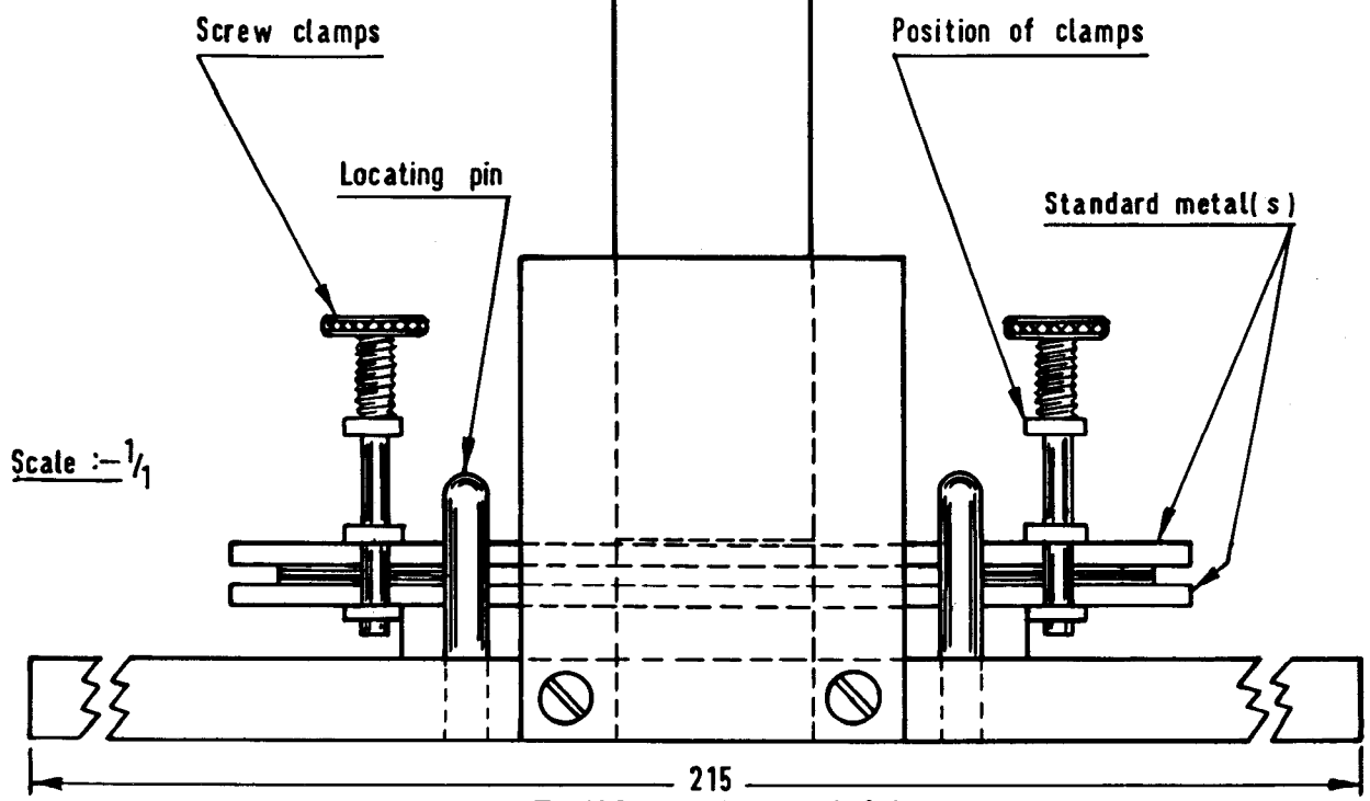
SUPPORT JIG - SIDE VIEW
