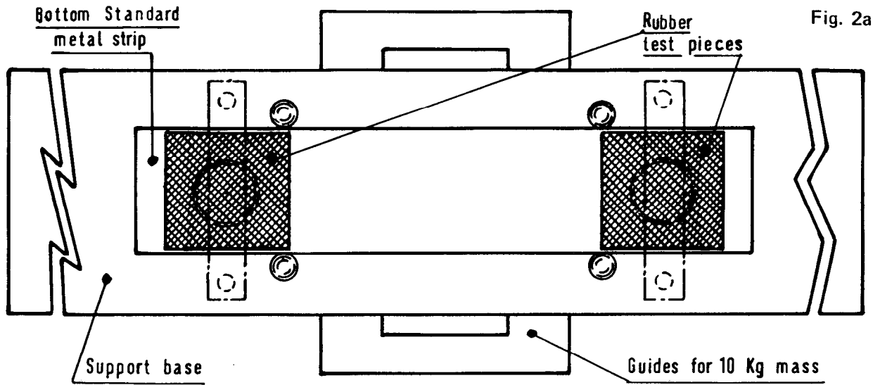
PLAN VIEW WITH CLAMPS, TOP STD. METAL STRIP & 10 Kg MASS REMOVED
