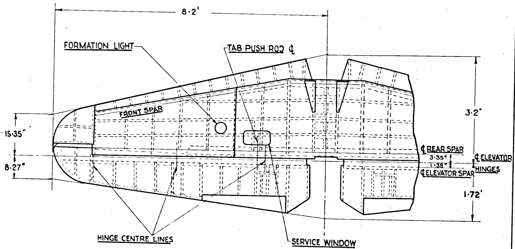
FIG.14 HORIZONTAL TAIL PLANE CONSTRUCTION DIAGRAM. SCALE 1/20.
